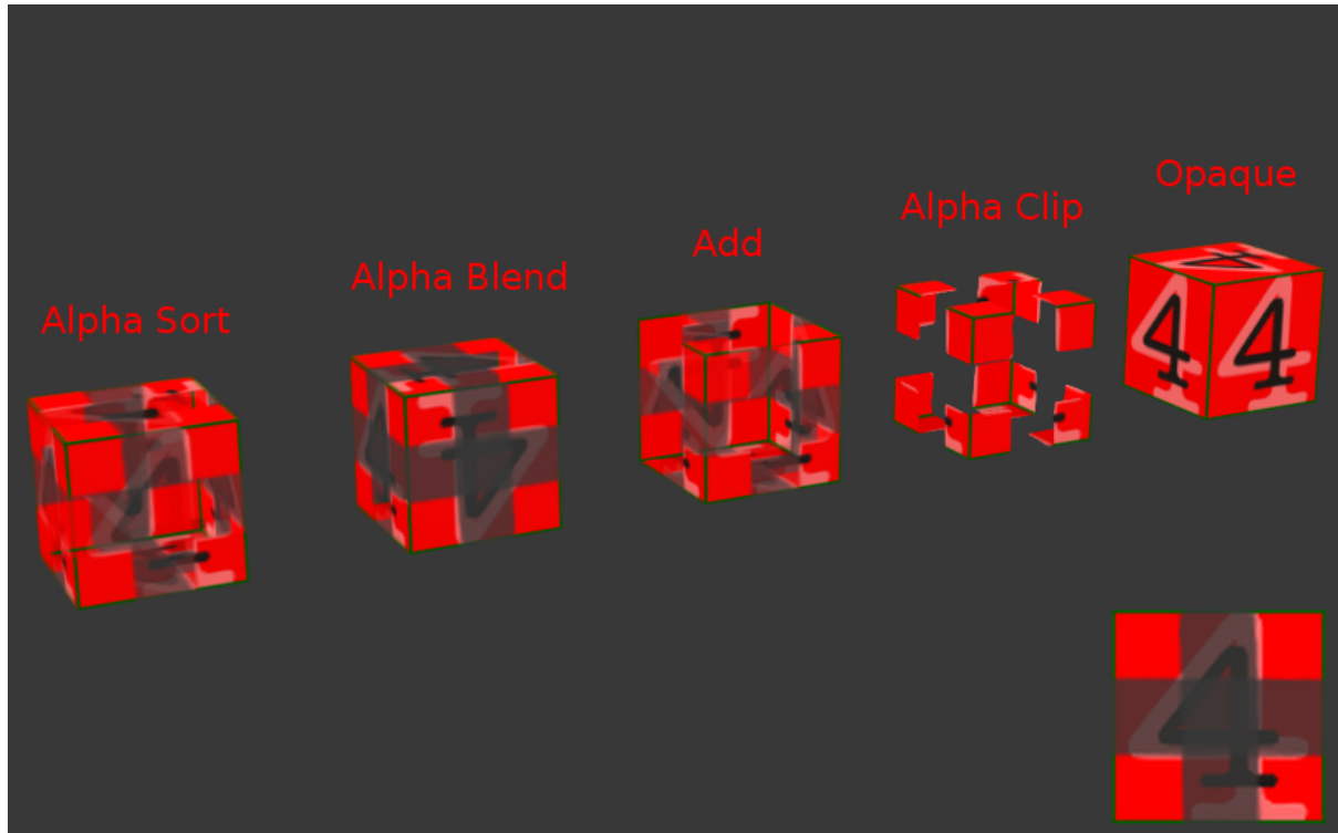
Figure 15.2: The engine supports all of the transparency types available in Blender.
